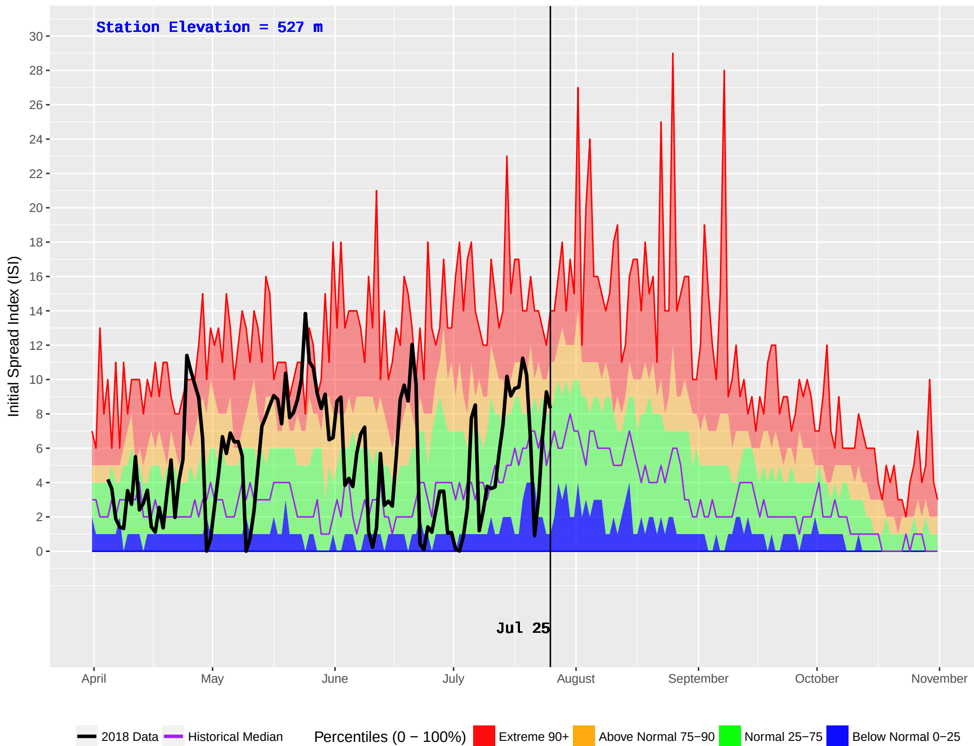
SALMON ARM (346) : Historical (1976–2016) and Current (2018) Noon Initial Spread Index (ISI)
