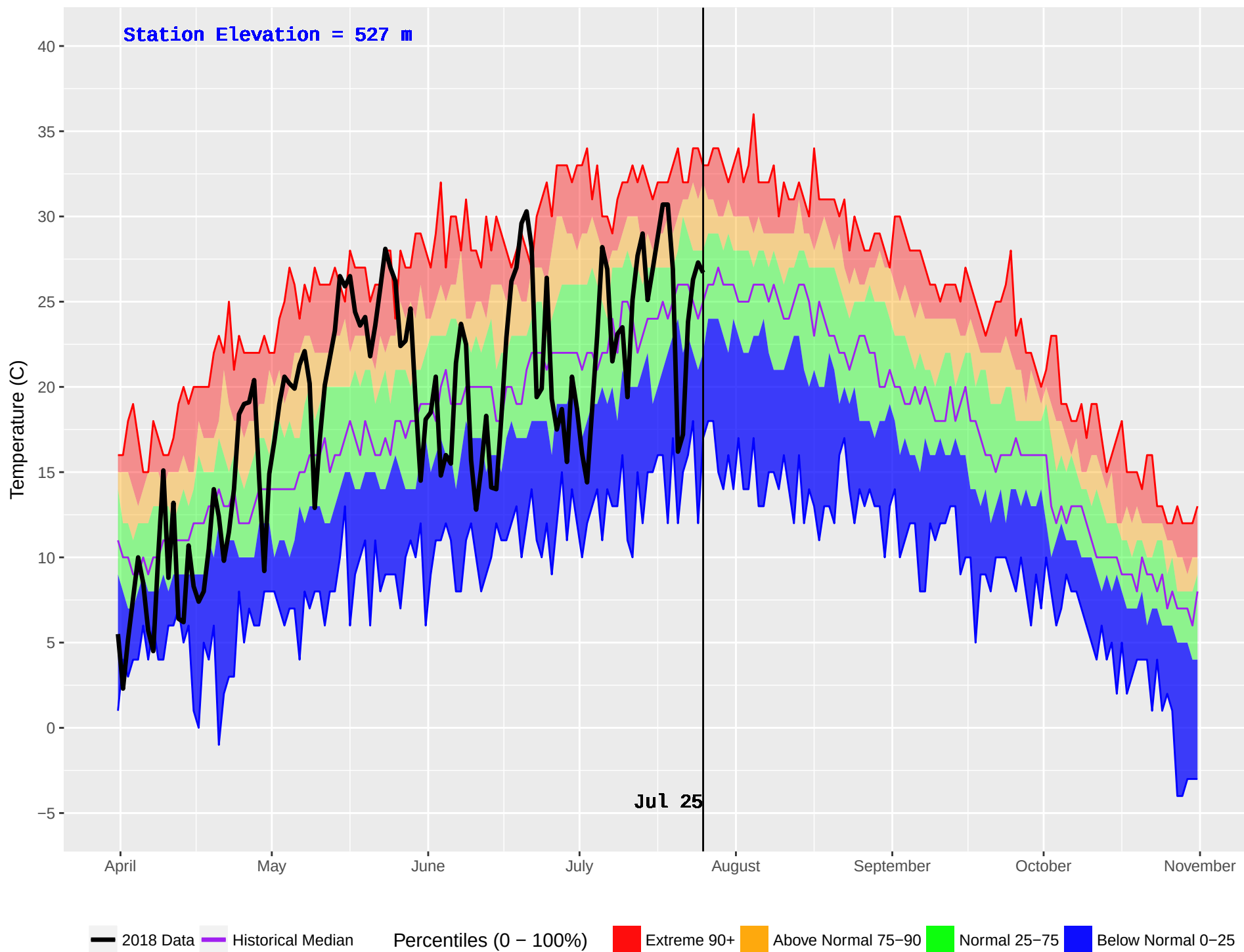
SALMON ARM (346) : Historical (1976–2016) and Current (2018) Noon Temperature
