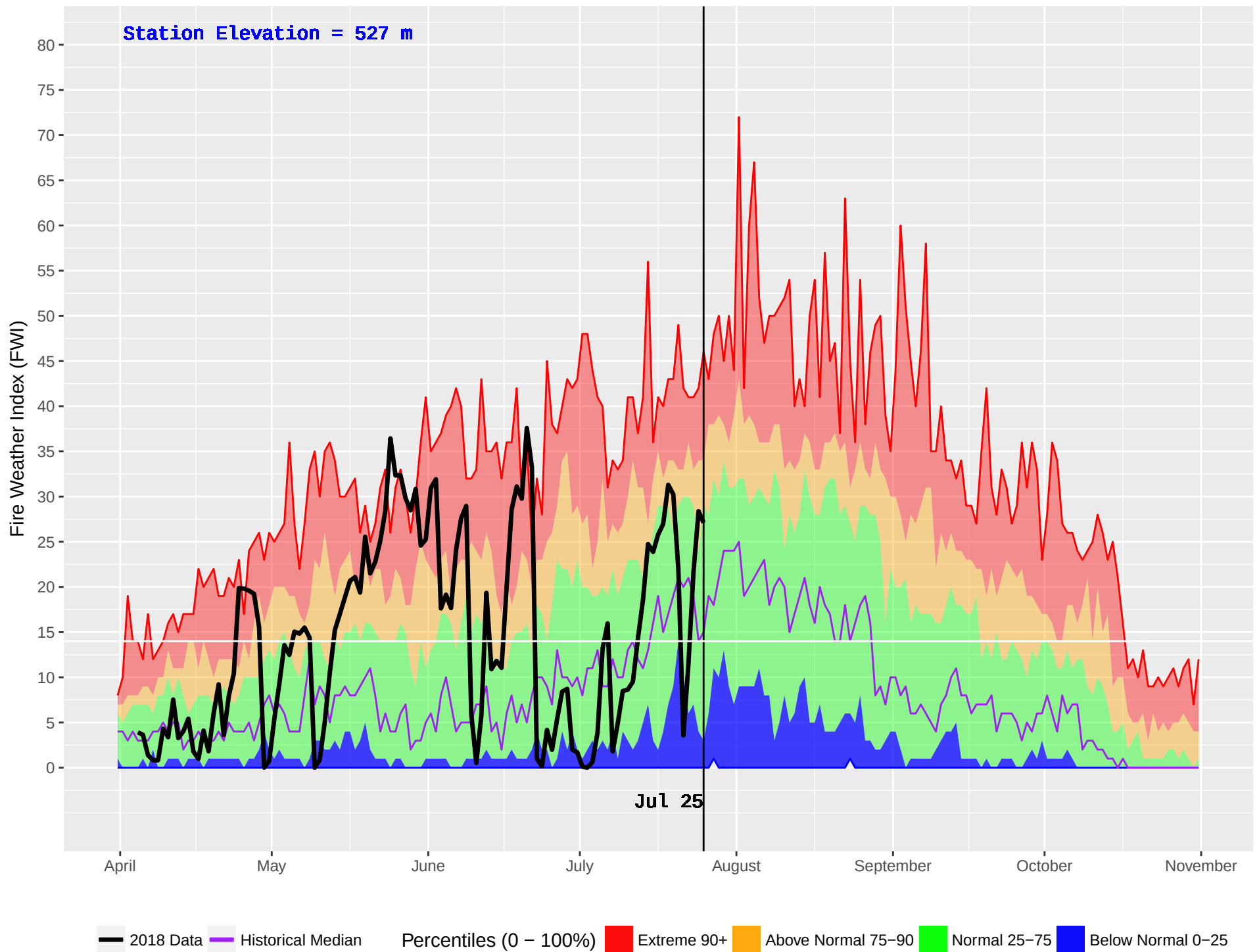
SALMON ARM (346) : Historical (1976–2016) and Current (2018) Noon Fire Weather Index (FWI)
