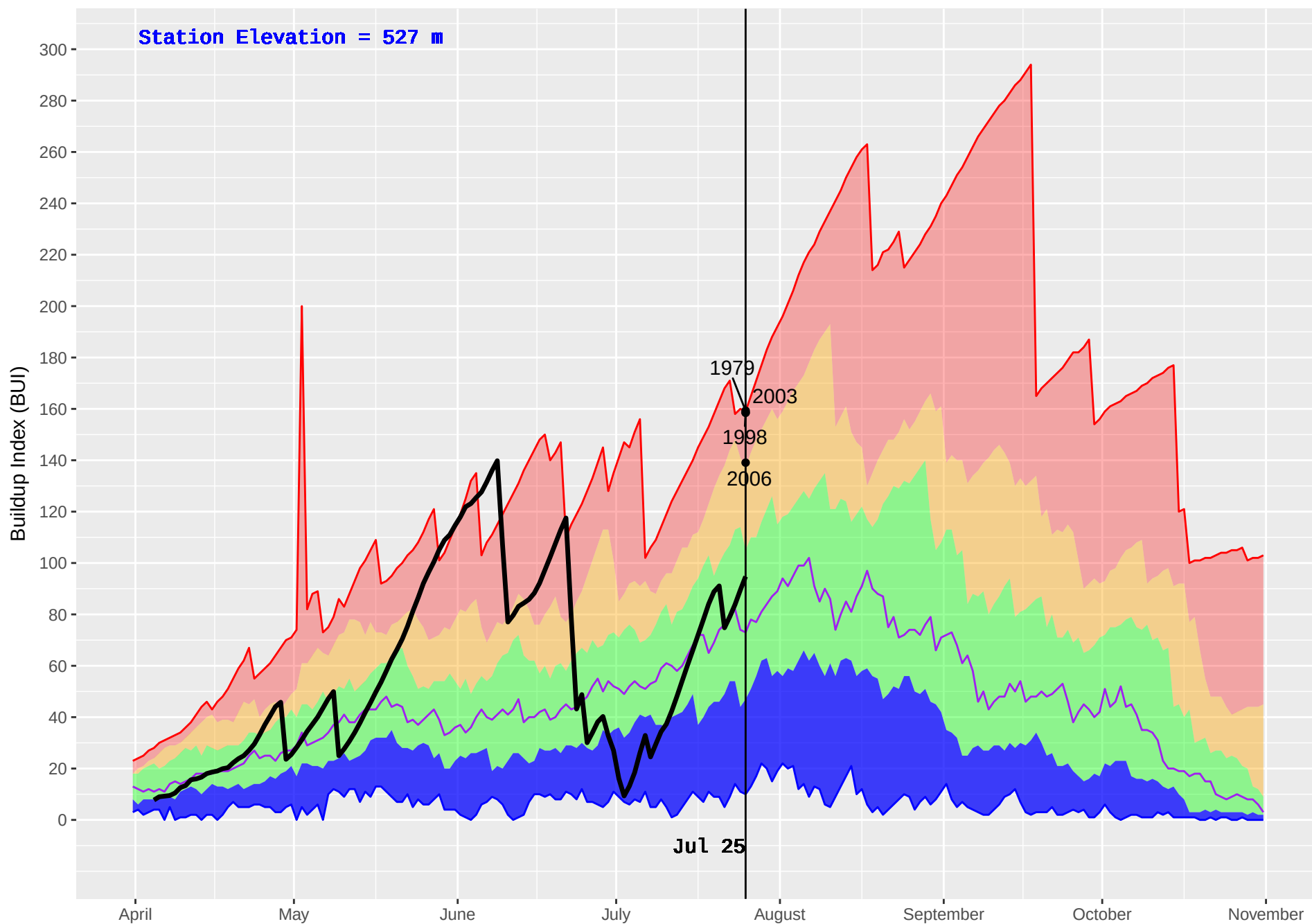
SALMON ARM (346) : Historical (1976–2016) and Current (2018) Noon Buildup Index (BUI)
