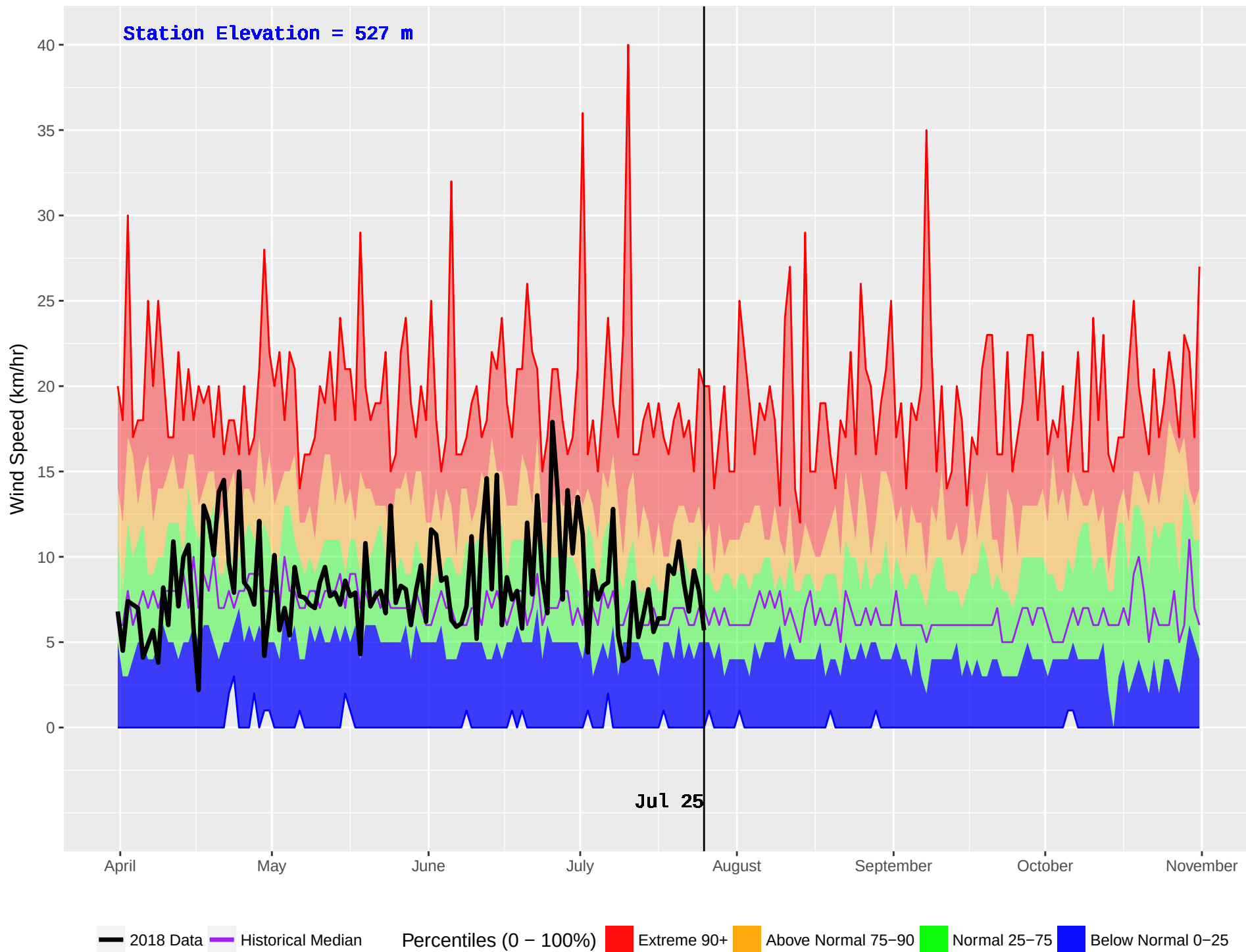
SALMON ARM (346) : Historical (1976–2016) and Current (2018) Noon Wind Speed
