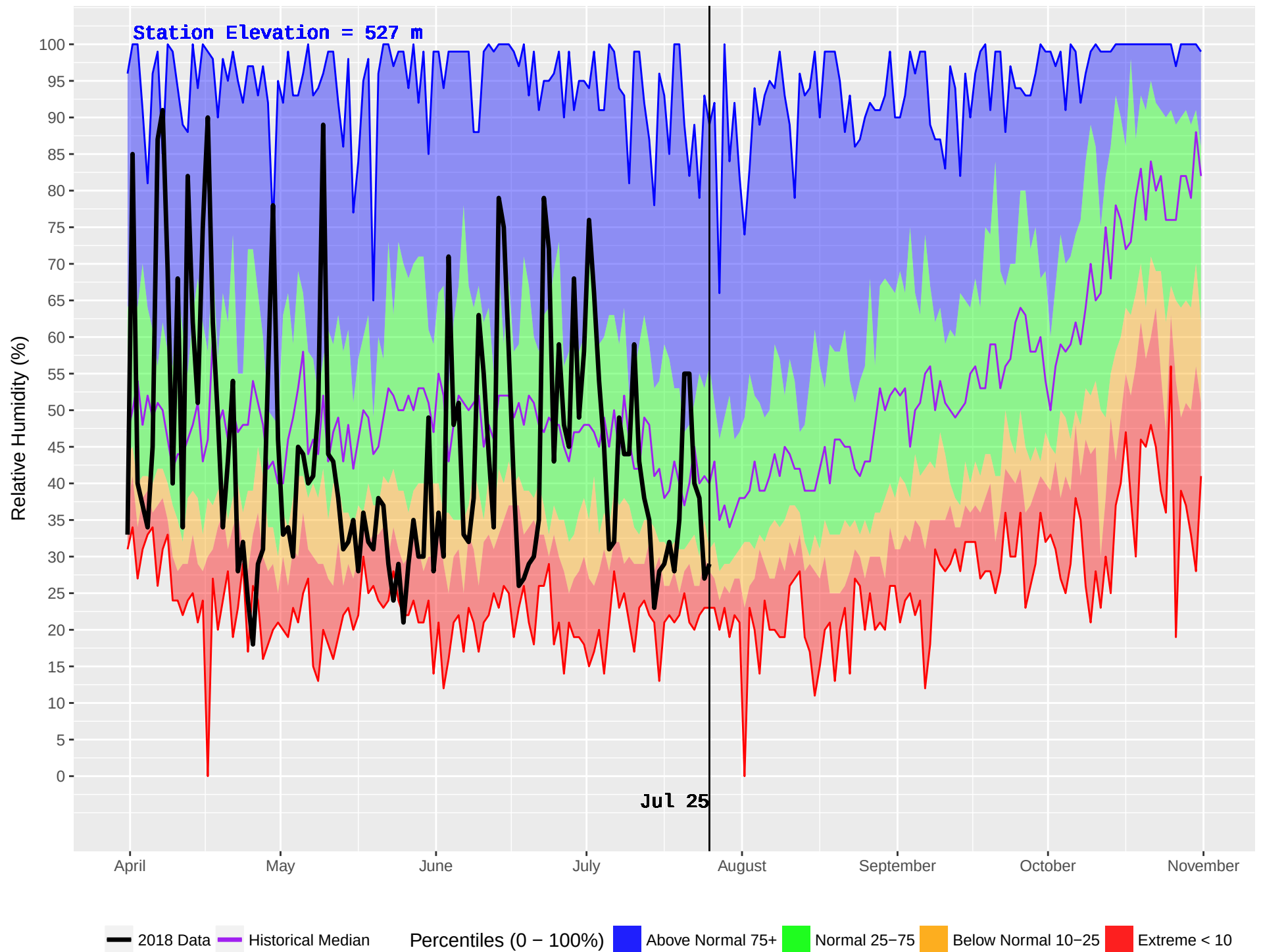
SALMON ARM (346) : Historical (1976–2016) and Current (2018) Noon Relative Humidity
