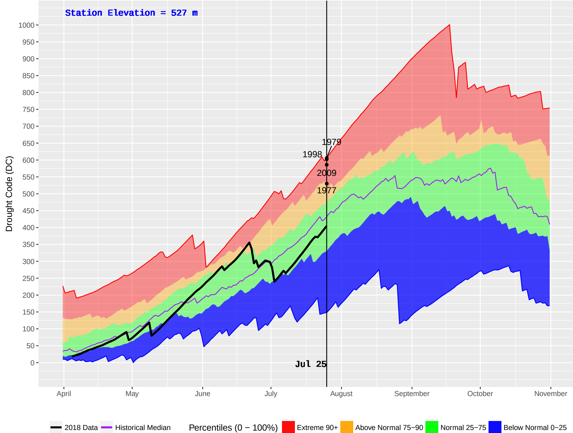
SALMON ARM (346) : Historical (1976–2016) and Current (2018) Noon Drought Code (DC)
